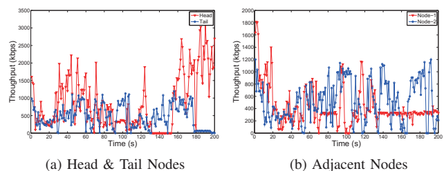
Fig. 1. Channel Diversity
