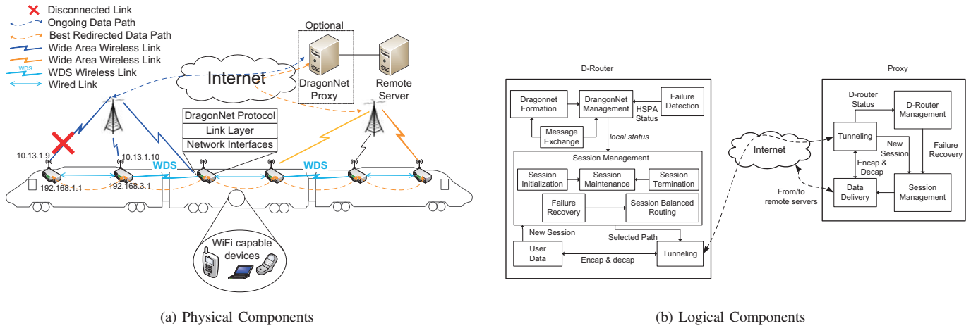
Fig. 2. DragonNet Architecture
